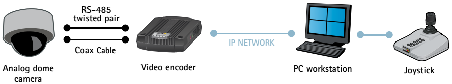
Figure 5.4a An analog PTZ dome camera can be controlled via the video encoder's serial port (e.g., RS-485), making it possible to remotely control it over an IP network.
