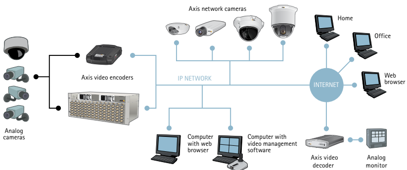
Figure 5.1a An illustration of how analog video cameras and analog monitors can be integrated with a network video system using video encoders and decoders.
