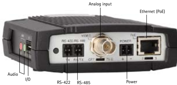
Figure 5.1b A one-channel, standalone video encoder with audio, I/O (input/output) connectors for controlling external devices such as sensors and alarms, serial ports (RS-422/485) for controlling PTZ analog cameras and Ethernet connection with Power over Ethernet support.
